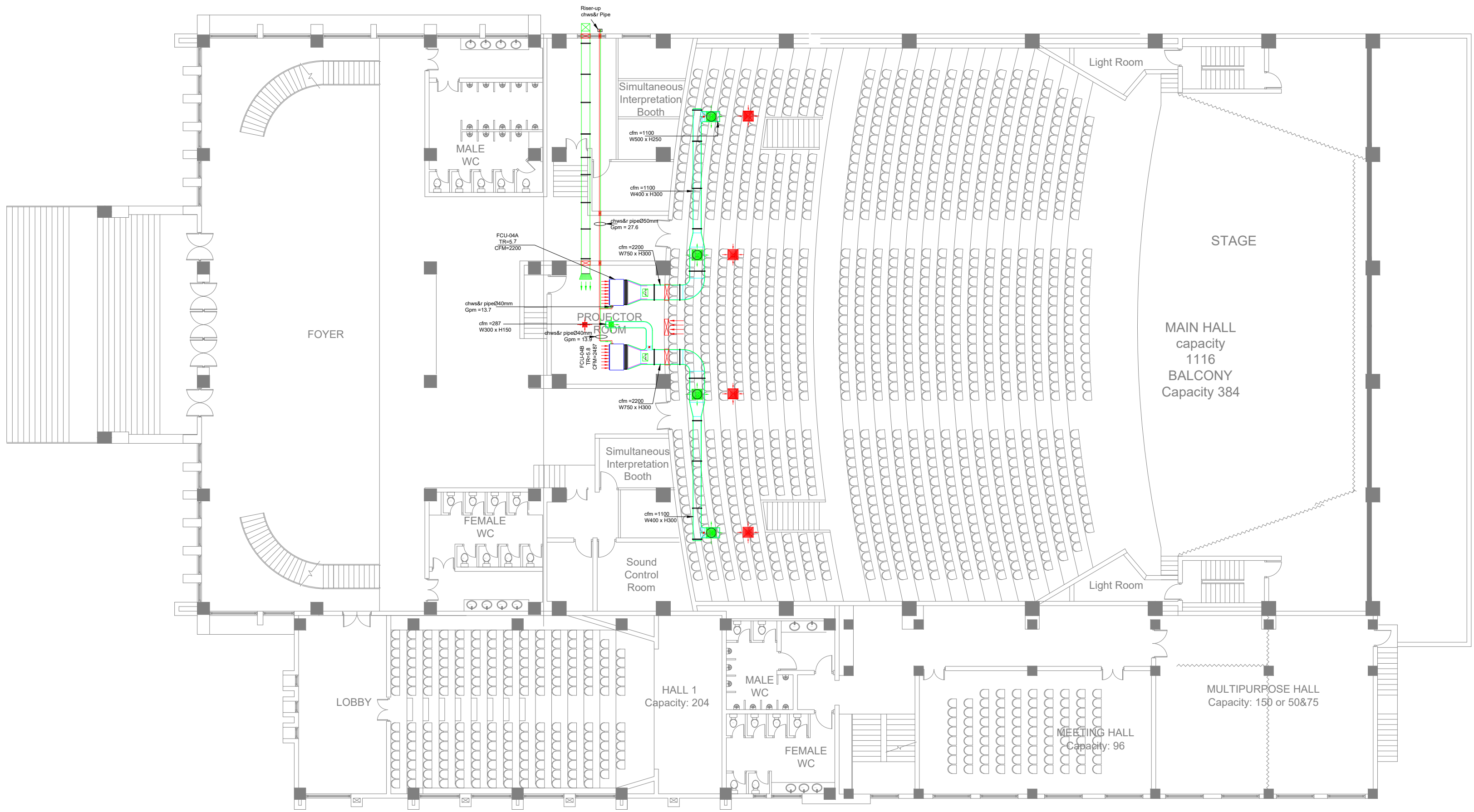
FIRST FLOOR PLAN Area: 2473 Sq.m. Scale= 1:250
